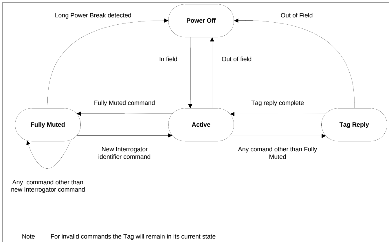
Figure M2-28 : Tag state transition diagram
