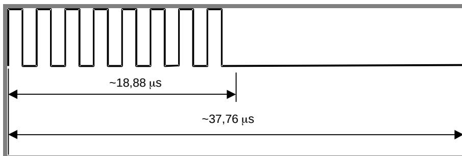
Figure M1-15 — Logic 0
