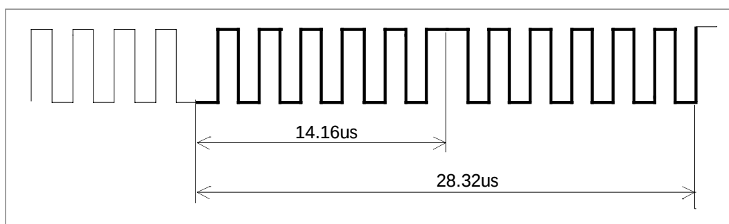
Figure M1-110 — End of signalling terminator coding
