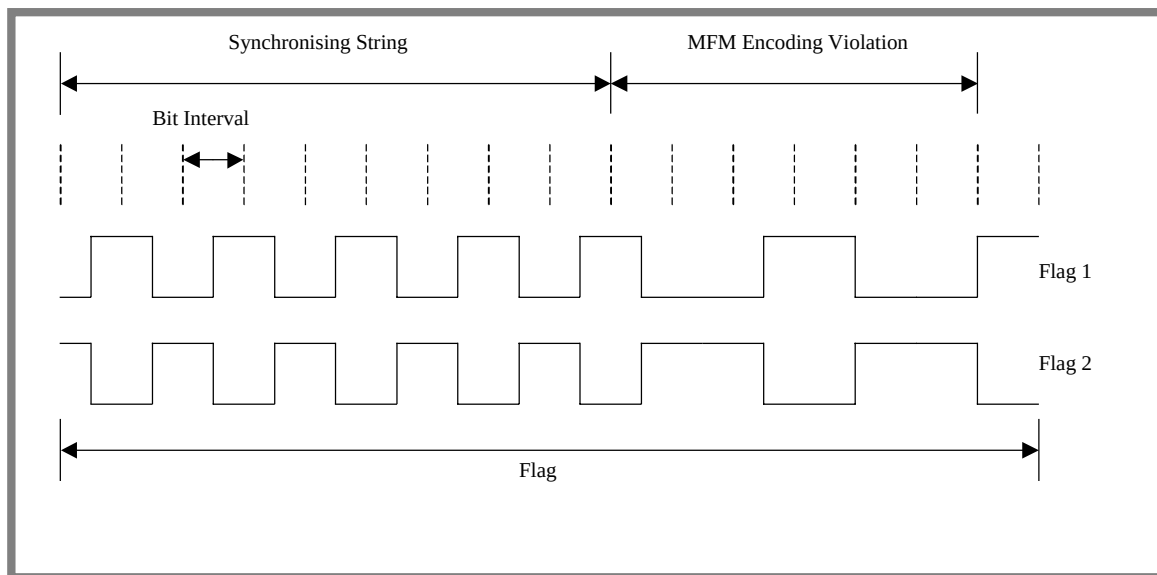
Figure M2-4 : Two possible reply flags
