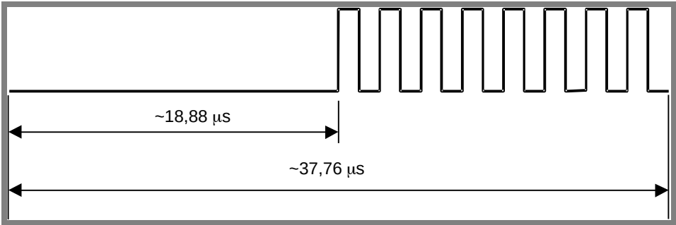
Figure M1-16 — Logic 1
