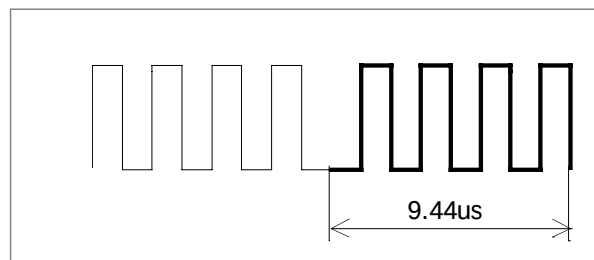
Figure M1-107 — Reply coding - binary 0
