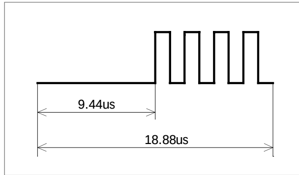
Figure M1-106 — Collision detection coding - binary 1
