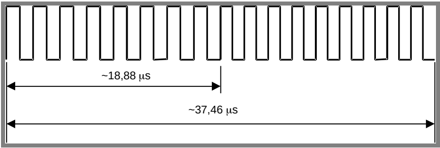
Figure M1-17 — Logic 0
