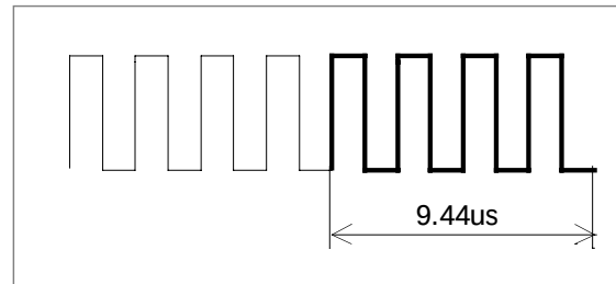
Figure M1-108 — Reply coding - binary 1
