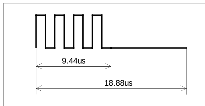
Figure M1-105 — Collision detection coding - binary 0
