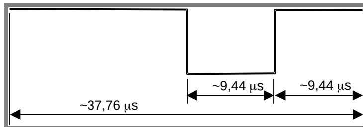
Figure M1-13 — End of frame for either mode
