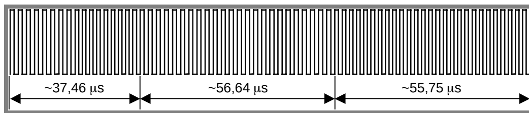
Figure M1-22 — End of frame when using 2 subcarriers
