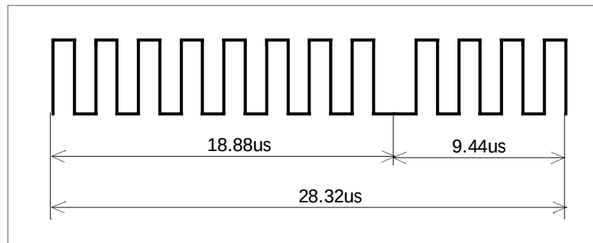
Figure M1-104 — Leader coding
