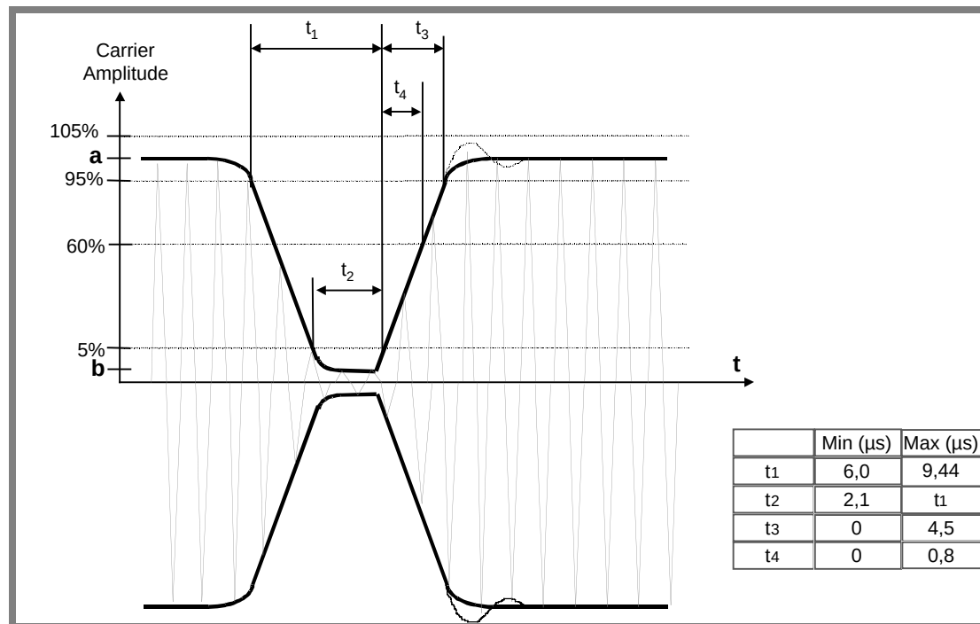
Figure M1-5 — Modulation of the carrier for 100% ASK
