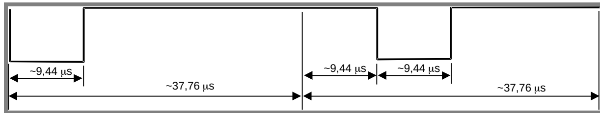
Figure M1-12 — Start of frame of the 1 out of 4 mode
