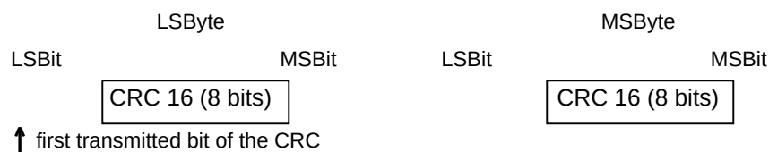
Figure M1-27— CRC bits and bytes transmission rules
