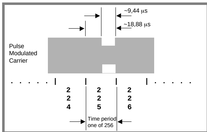
Figure M1-8 — Detail of one time period
