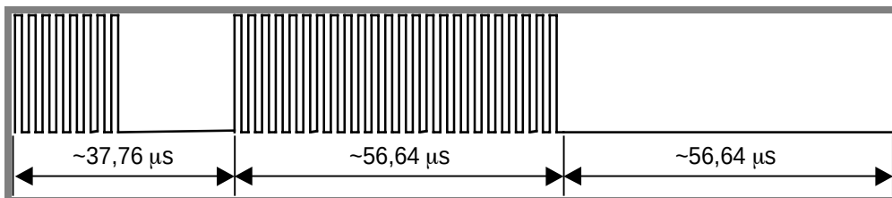
Figure M1-21— End of frame when using one subcarrier
