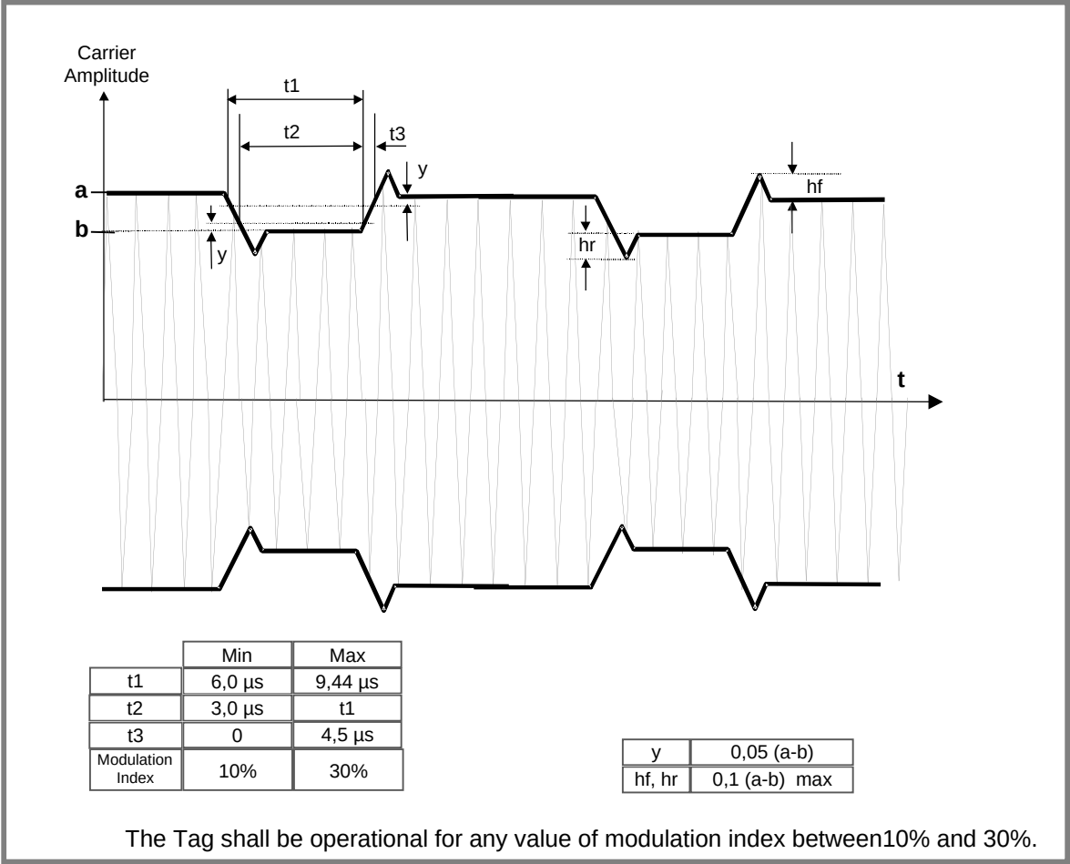
Figure M1-6 — Modulation of the carrier for 10% ASK
