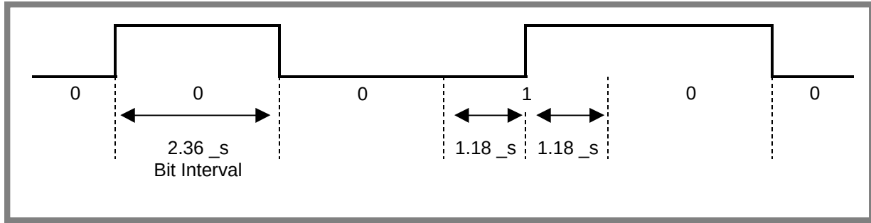
Figure M2-6 : Command MFM encoding and timing of binary 000100
