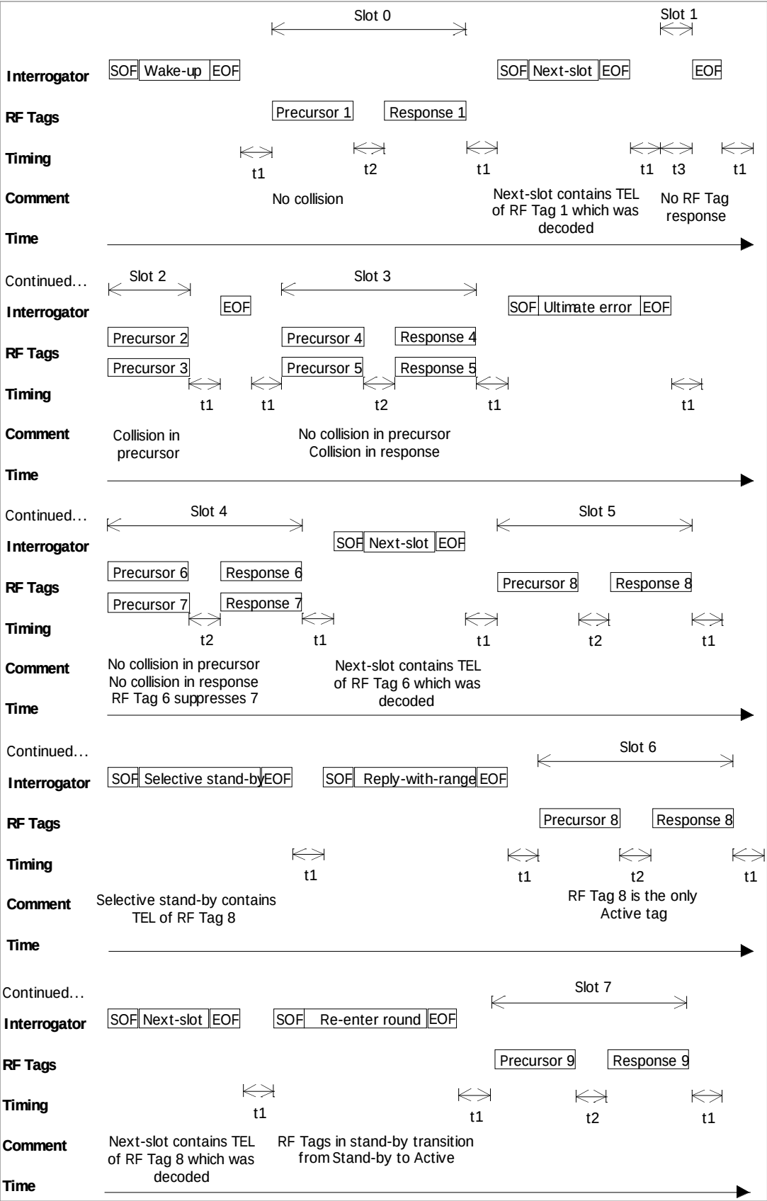
Figure M1-95 — Slotted terminating adaptive round
