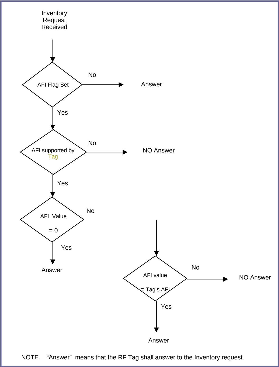
Figure M1-26 — RF Tag decision tree for AFI
