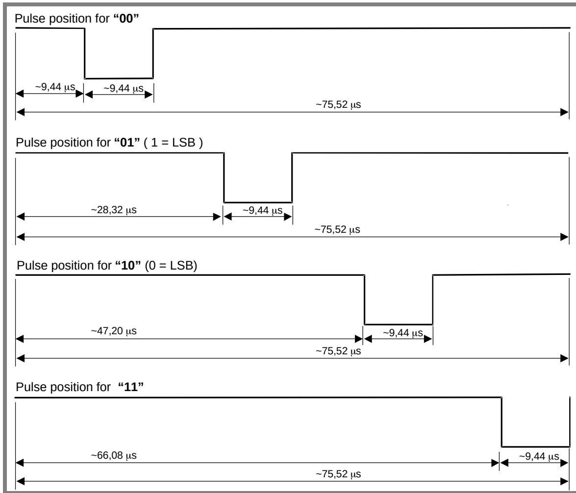
Figure M1-9 — 1 out of 4 coding mode
