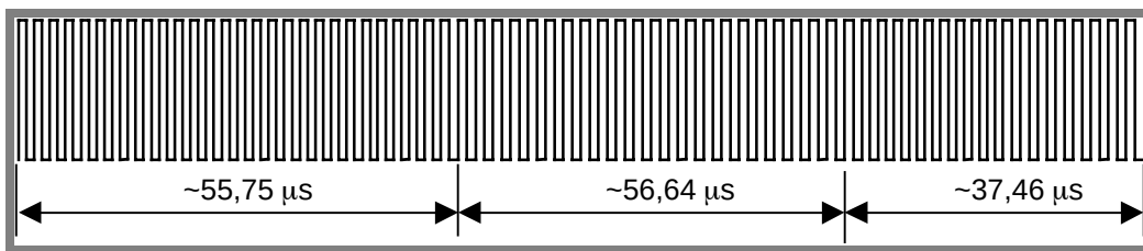
Figure M1-20 — Start of frame when using two subcarriers
