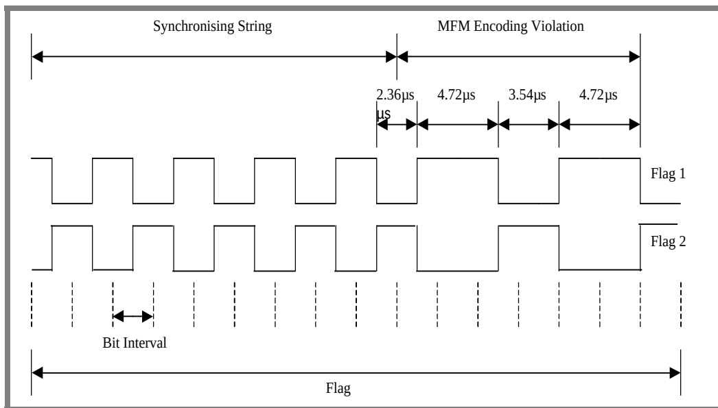
Figure M2-7 : MFM encoding and timing for two possible command flags
