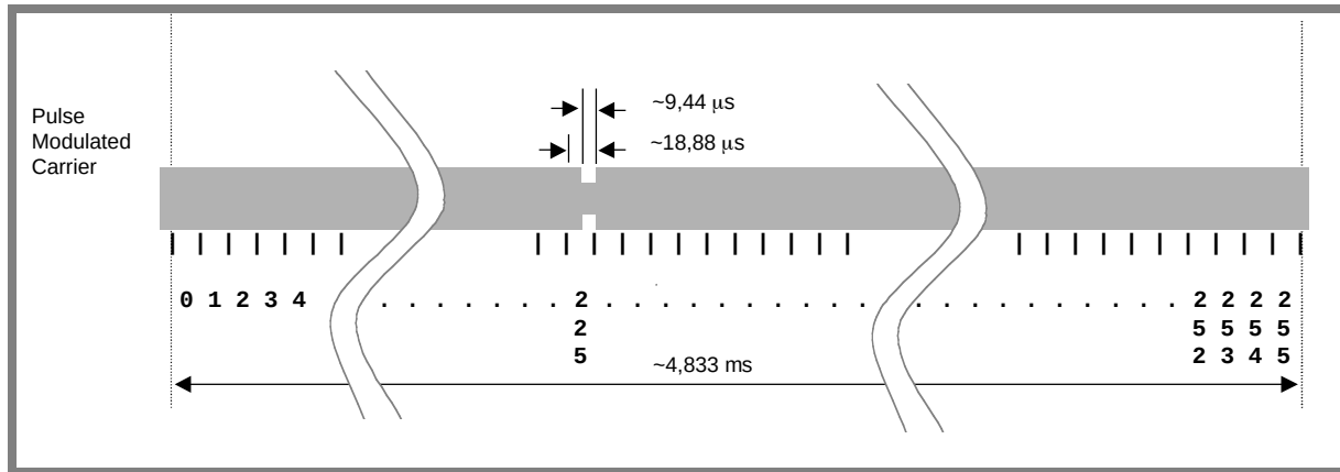
Figure M1-7 — 1 out of 256 coding mode
