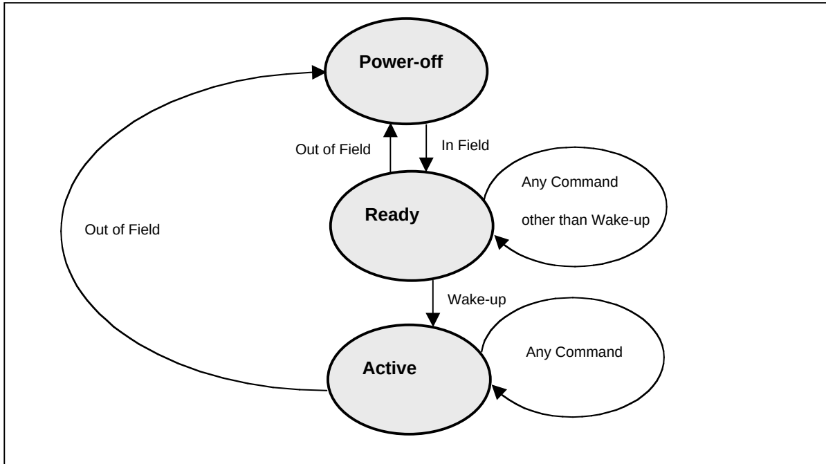
Figure M1-93 — Tag states in non-slotted non-terminating multiple Tag reading protocol
