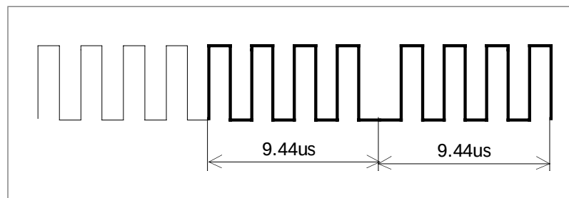
Figure M1-109 — Reply coding - “10”
