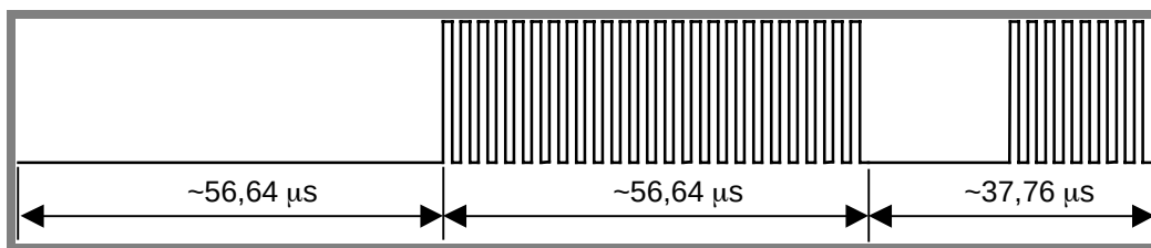
Figure M1-19 — Start of frame when using one subcarrier
