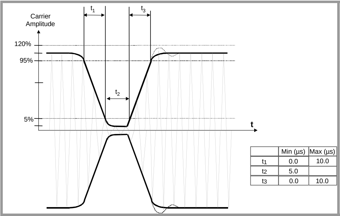
Figure M2-29 : Interrogator powering field breaks
