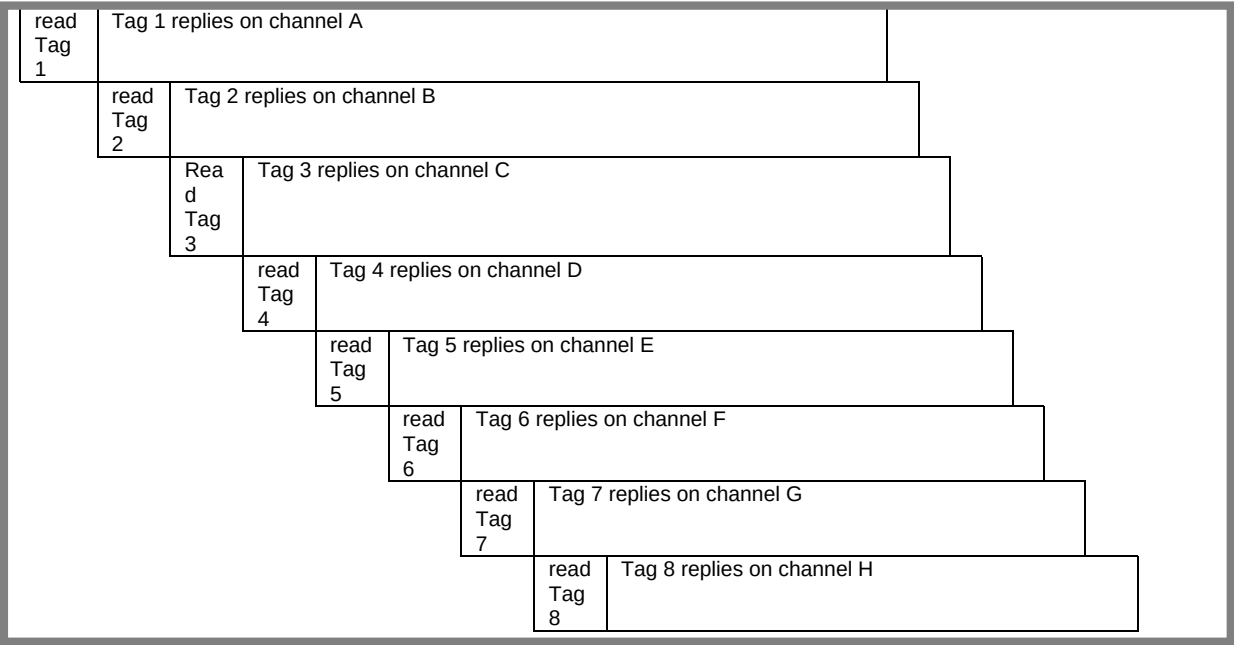
Figure M2-33 : Reading data from 8 Tags
