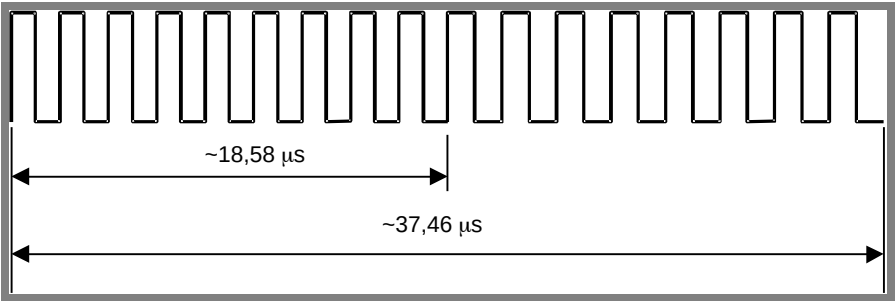
Figure M1-18 : logic 1
