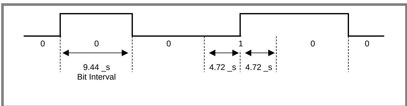
Figure M2-10 : Reply MFM encoding and timing of binary 000100
