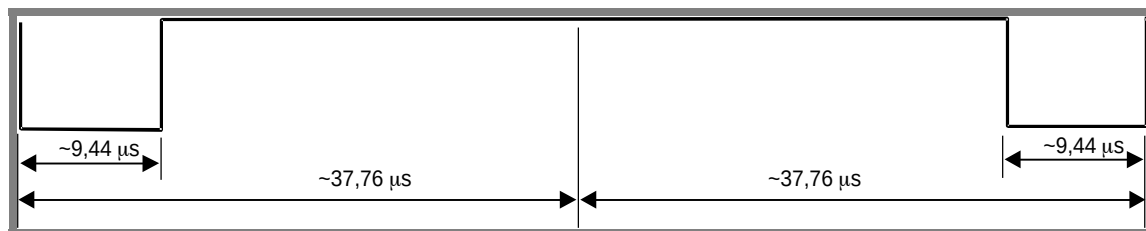
Figure M1- 11 — Start of frame of the 1 out of 256 mode
