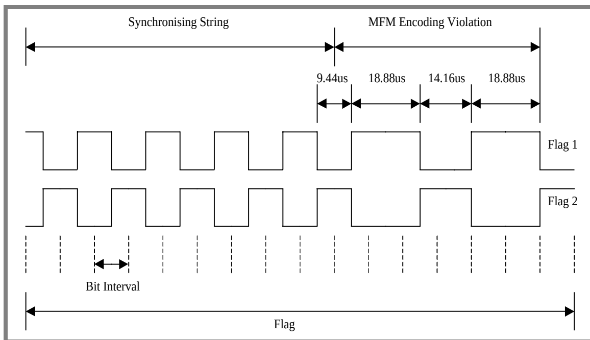
Figure M2-11 : MFM encoding and timing for two possible reply flags
