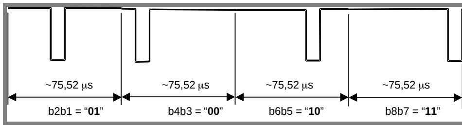
Figure M1-10 — 1 out of 4 coding example
