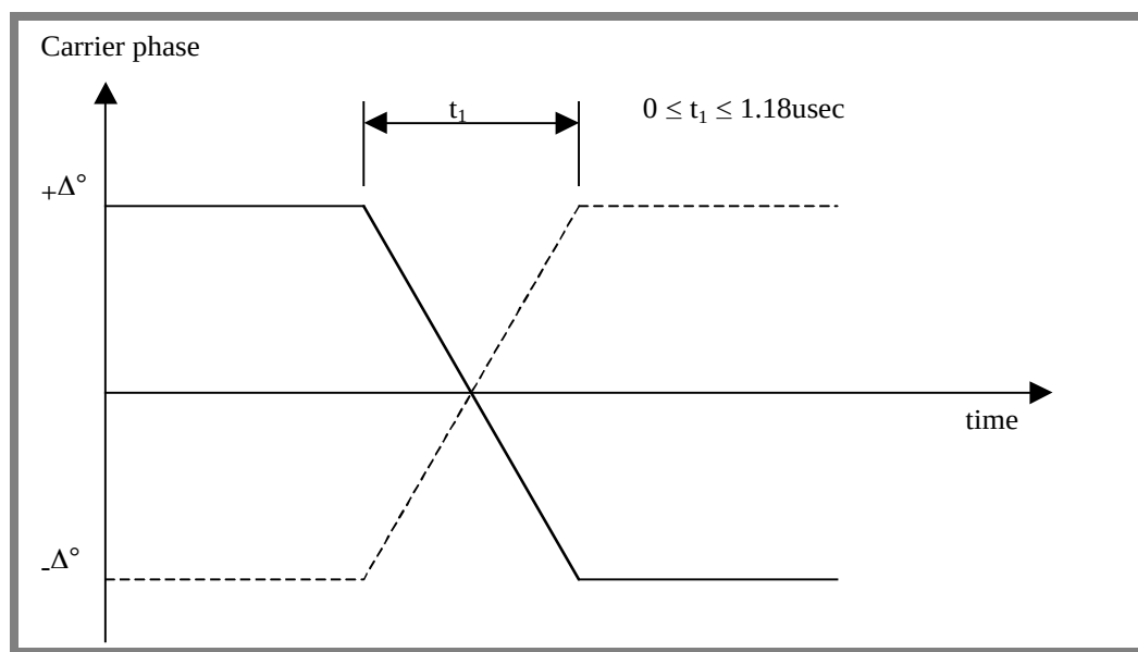
Figure M2-5: Command modulation scheme
