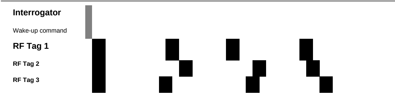
Figure M1-92 — Example of RF Tag response in non-slotted non-terminating multiple Tag reading protocol
